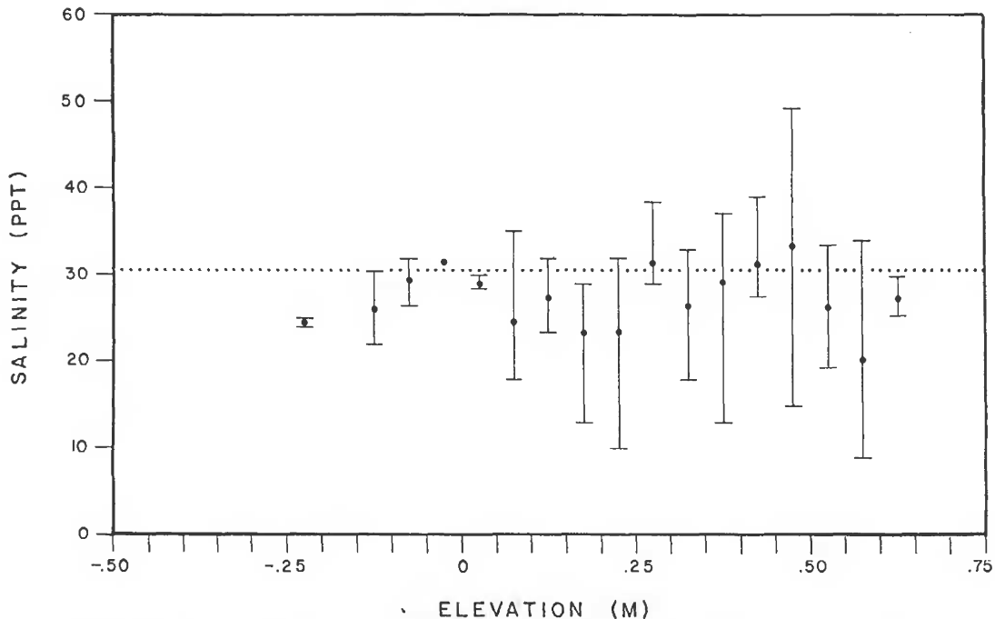
Figure 8. Salinity of water extracted from sediment samples collected within 0.05-m intervals. Average salinities are represented by dots. Vertical bars show the range of salinities measured within each interval. Salinity of tidal water flooding the study site is shown as a dotted line.
